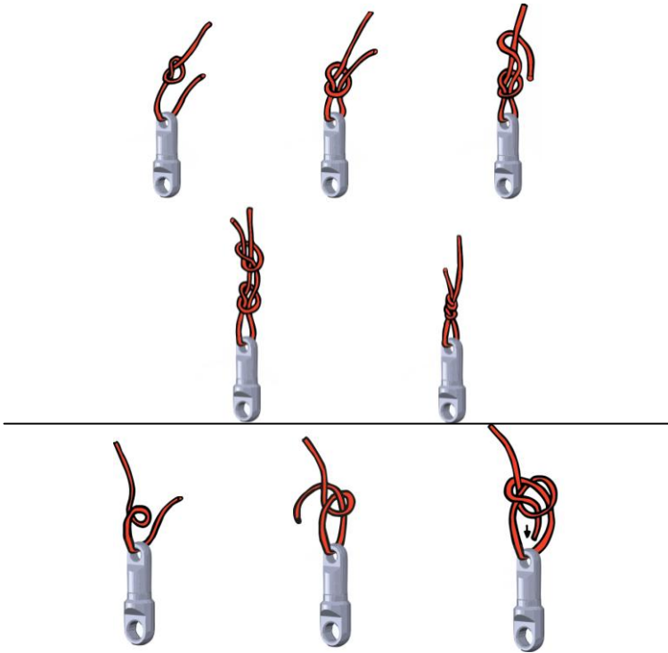
Illustration 7 and 8: Fisherman's knot and bowline
